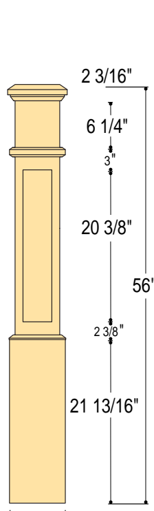
7 1/2" C-4890 Mission 6" Top Sq. 7 1/2" Bottom Sq.
