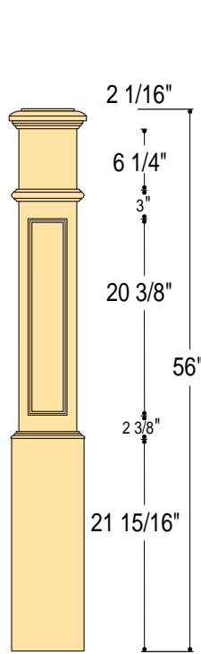
7 1/2" C-4891 Recessed Panel 6" Top Sq. 7 1/2" Bottom Sq.
