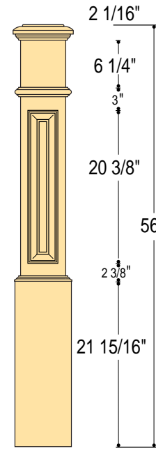
7 1/2" C-4892 True Raised Panel 6" Top Sq. 7 1/2" Bottom Sq.
