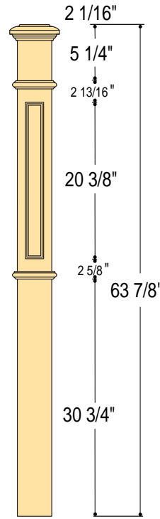
4 1/2" C-4691 Recessed Panel 4 1/2" Sq.
