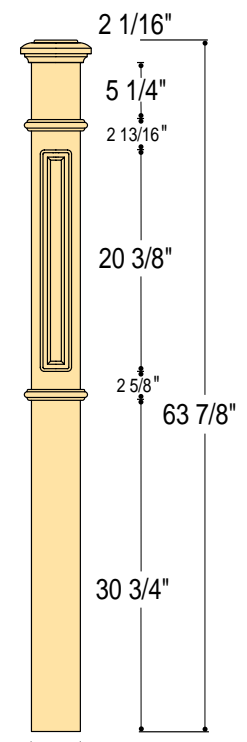
4 1/2" C-4697 Raised Panel 4 1/2" Sq.
