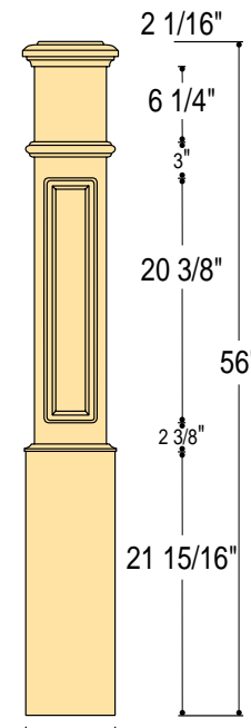
7 1/2" C-4097 Raised Panel 6" Top Sq. 7 1/2" Bottom Sq.
