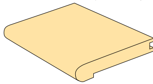
C-8590 Landing Tread 5-1/4" Wide
