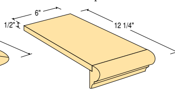
C-8972 6" x 11" Tread Cap with Nosing and Cove
