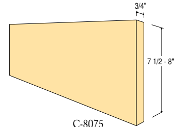
C-8075 Riser 3/4" x 7-1/2" and 8"
