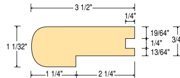
C-8090 - 3-1/2" Wide C-8590 - 5-1/4" Wide
