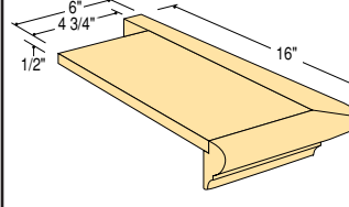
C-8071 4-3/4" x 11-1/2" Tread Cap with Mitered Return Nosing and Cove Left or Right (RH shown)
