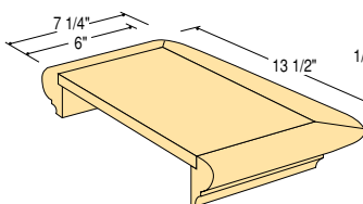
C-8971 6" x 11" Reversible Tread Cap with Mitered Return Nosing and Cove
