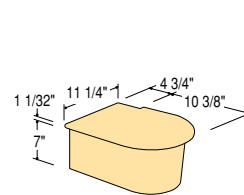
C-8011 Starting End Cap Left or Right (RH shown)
