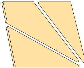
C-8370 Three Piece Winder Tread 1-1/32" x 36", 42" and 48" (RH shown)
