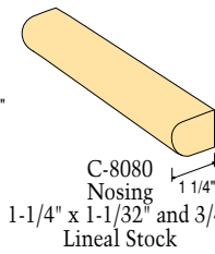
C-8080-12 MR C-8080-13 MR Coped Return Nosing 1-1/4" x 1-1/32" x 11-3/4" and 12-3/4"
