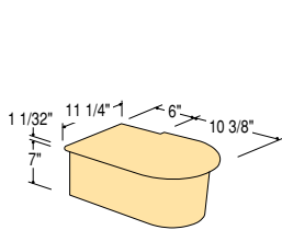
C-8911 Reversible Starting End Cap
