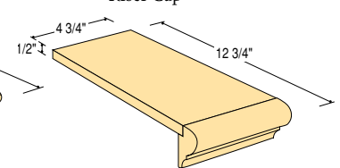
C-8072 4-3/4" x 11-1/2" Tread Cap with Nosing and Cove
