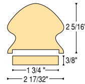
C-6005 P1 1 3/4" Plow with Fillet
