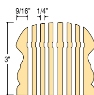
C-6716 Bending Rail
